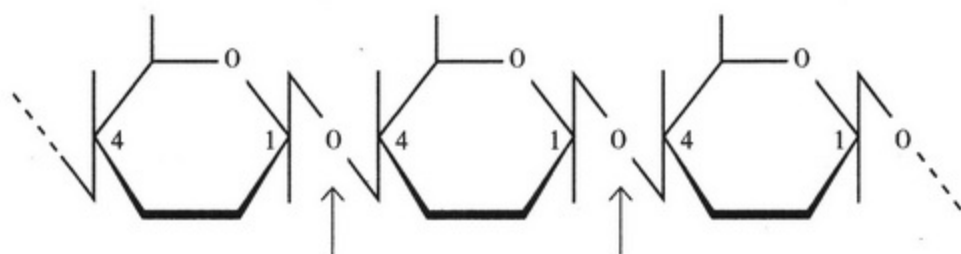
\beta(1 \rightarrow 4) 糖苷键
