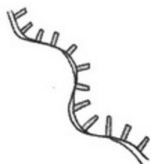
RNA
